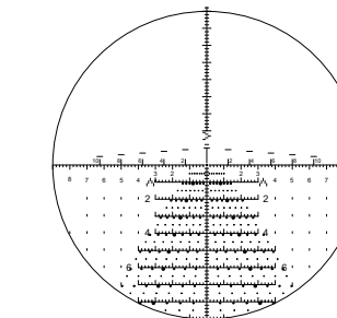
Tremor 3 Reticle*
